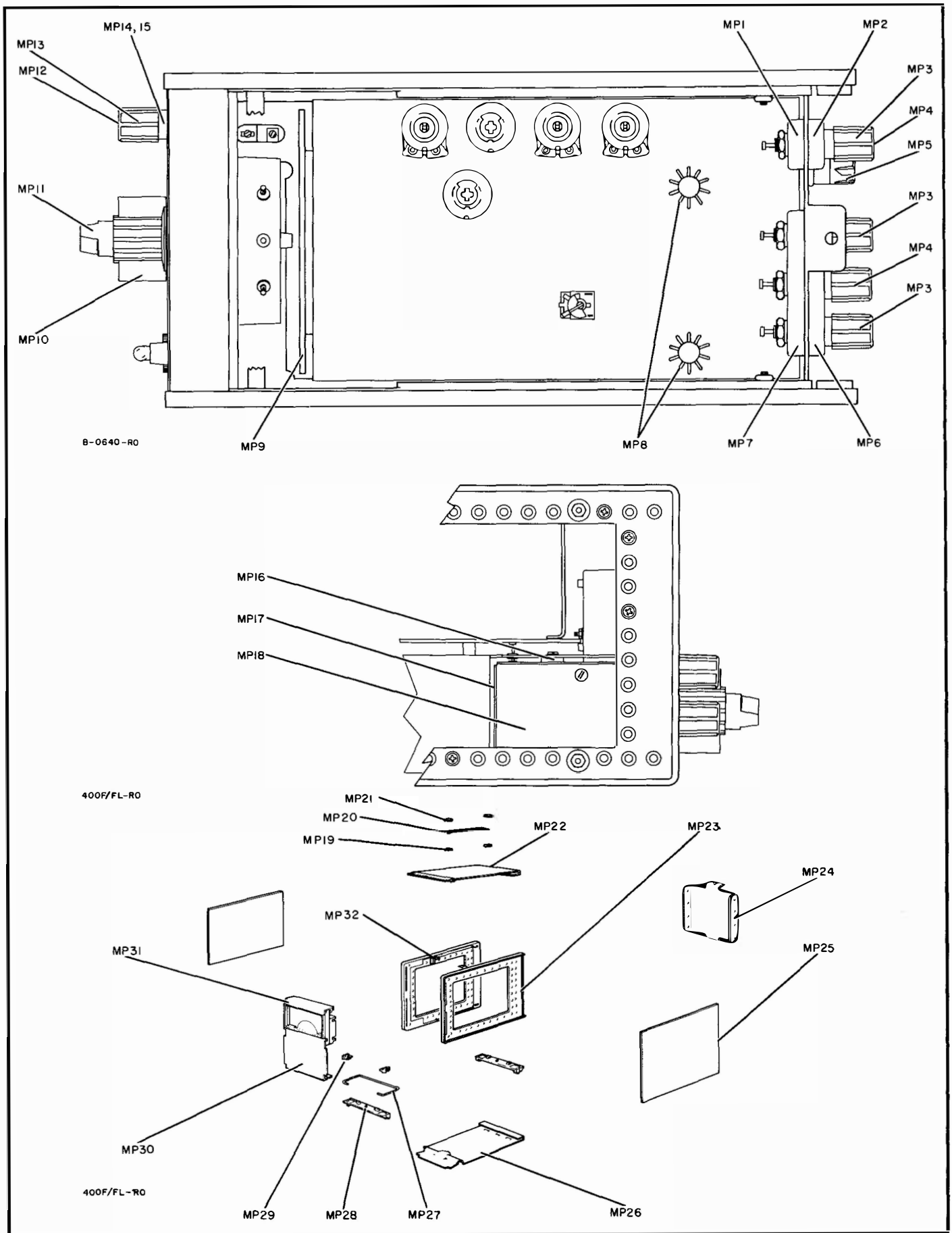
Figure 7-1. Location of Important Mechanical Parts
