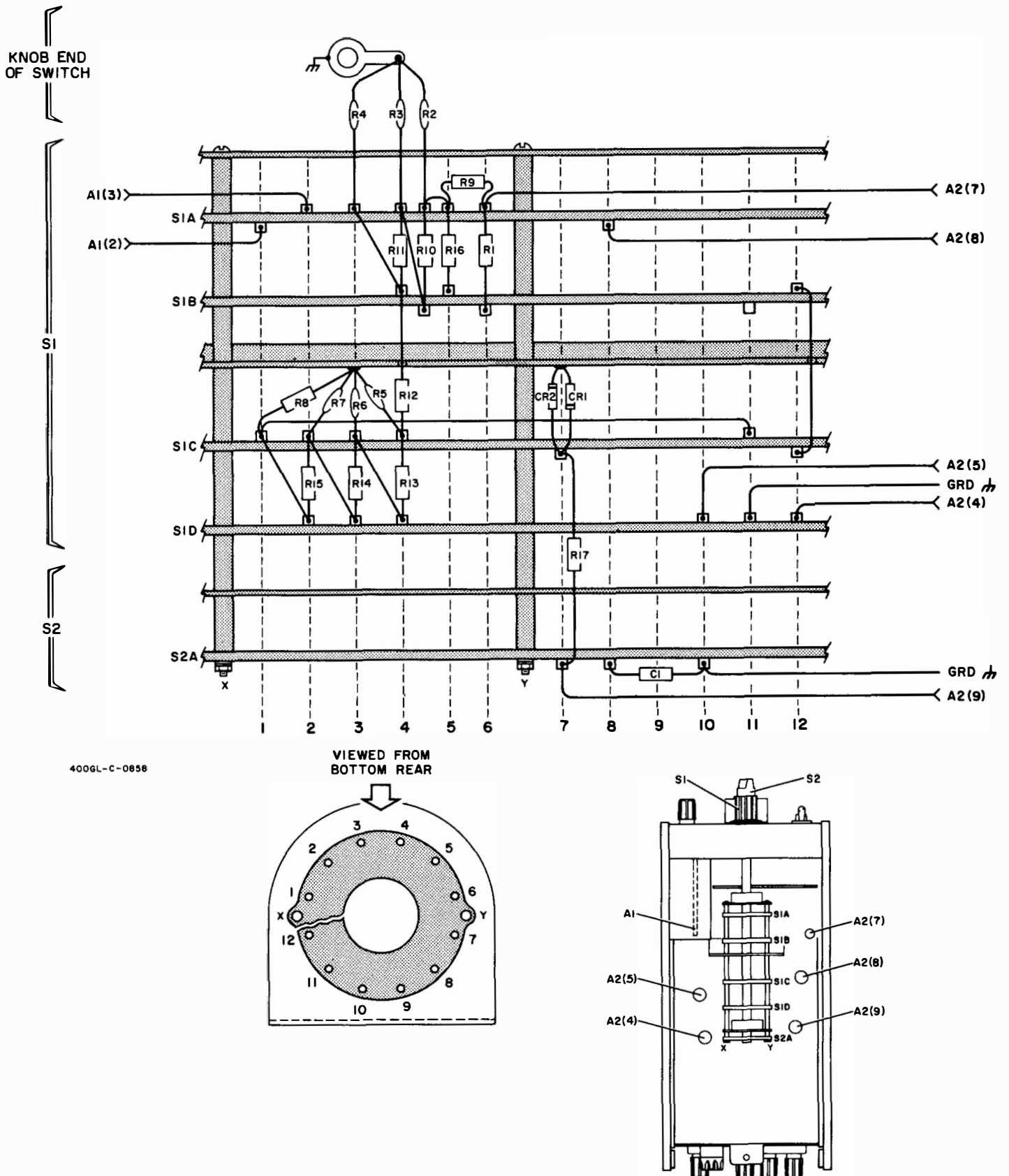
Figure 6-1. Model 400GL Range Switch
