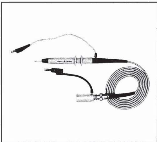
Figure 1-2. Model 11074A Voltage Divider Probe
