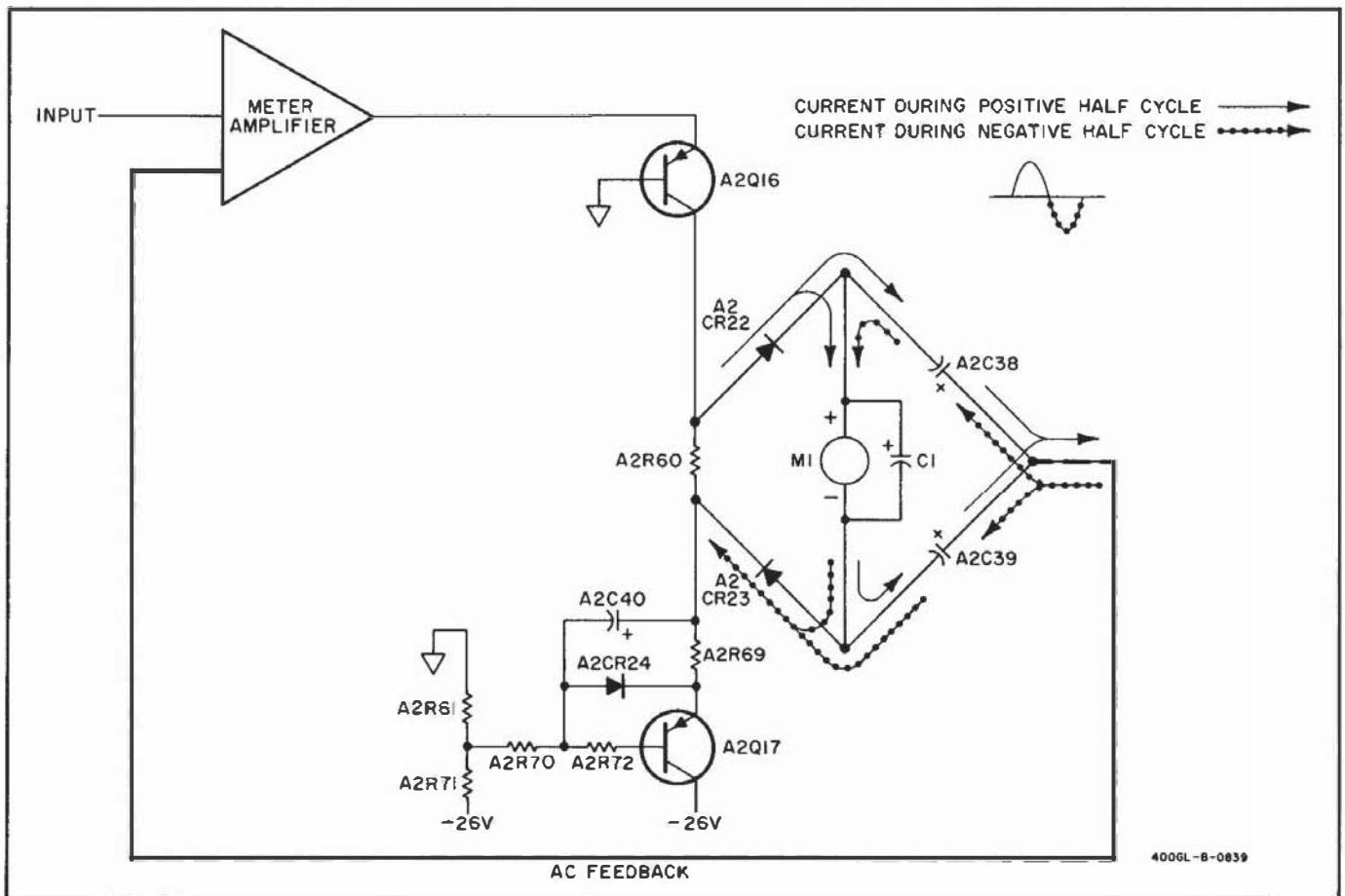
Figure 4-3. Simplified Diagram of Metering Circuit
