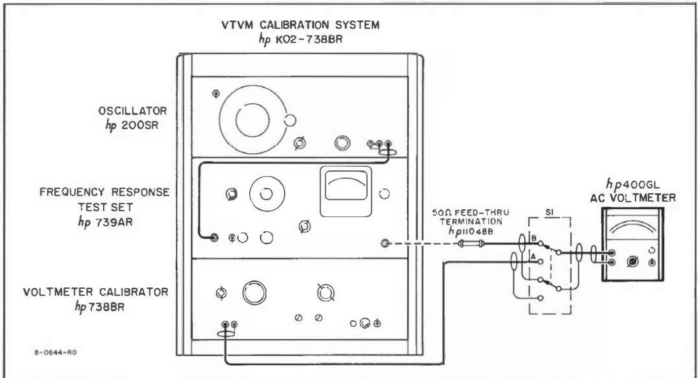
Figure 5-2. Alternate Accuracy and Frequency Response Check Setup
