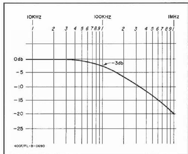
Figure 4-2. Filter Attenuation Characteristics
