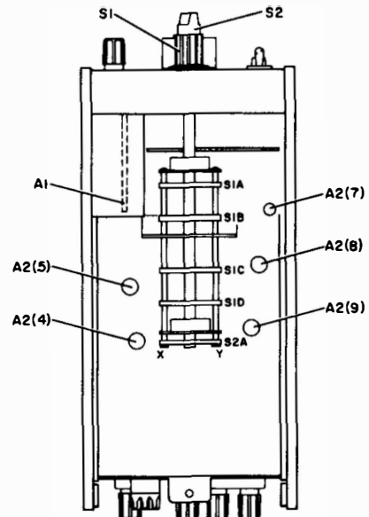
Figure 6-1. Model 400GL Range Switch
