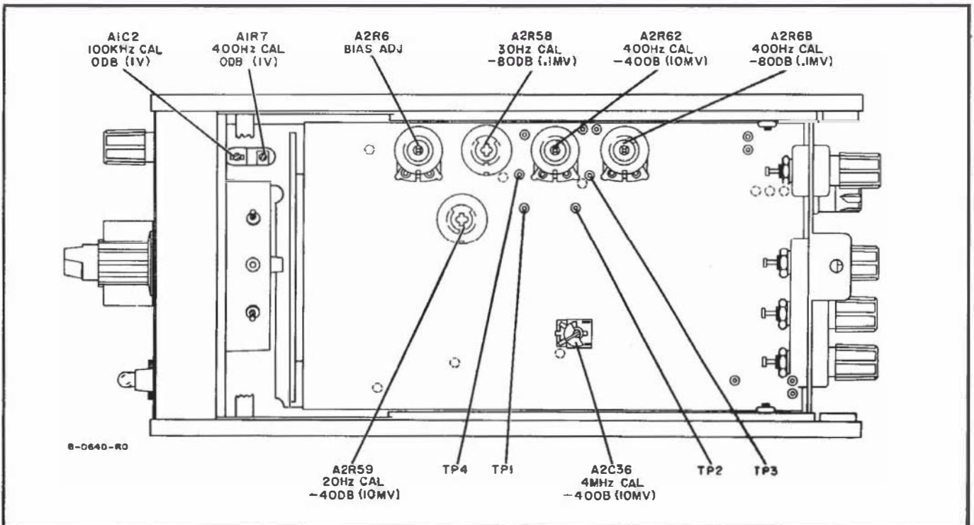
Figure 5-4. Location of Internal Adjustments
