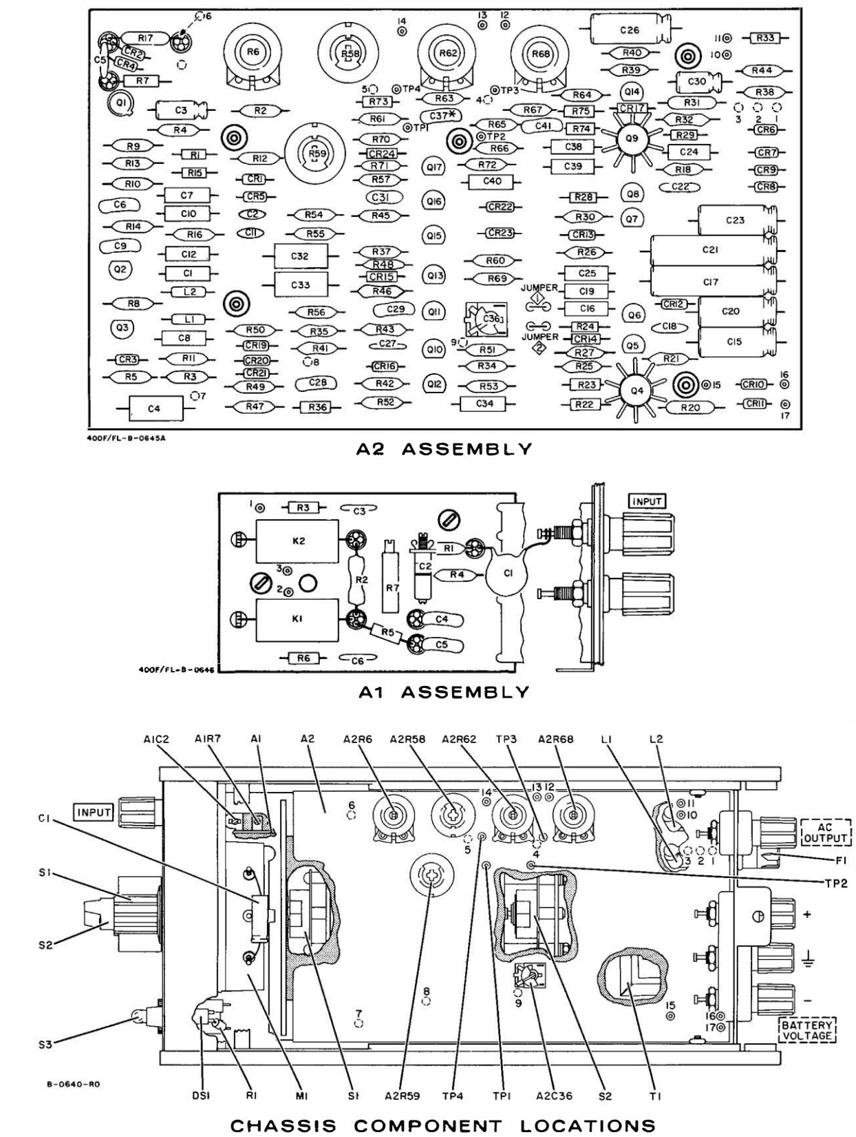
Figure 6-2. Model 400GL Component Location
