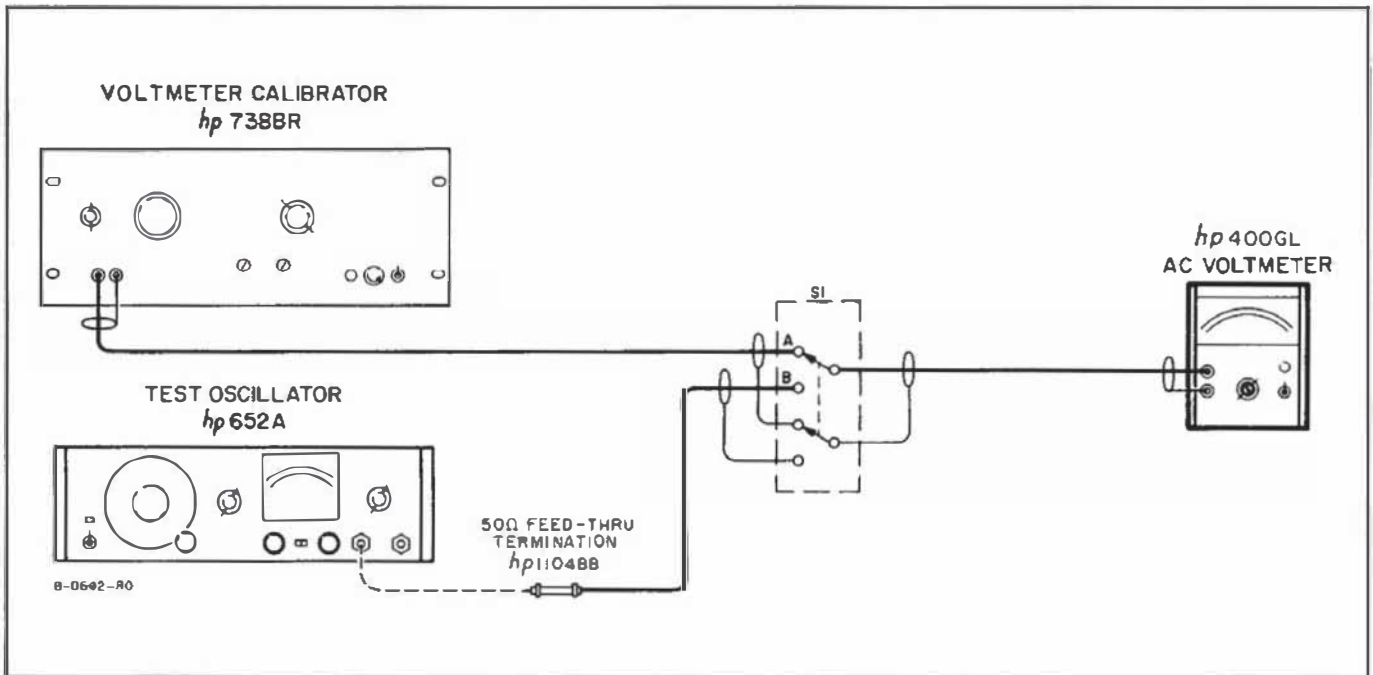
Figure 5-1. Accuracy and Frequency Response Check Setup
