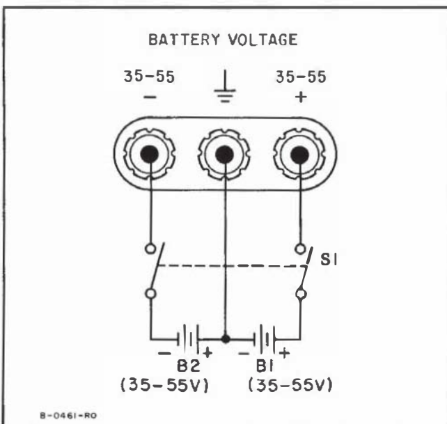
Figure 3-2. External Battery Connection
